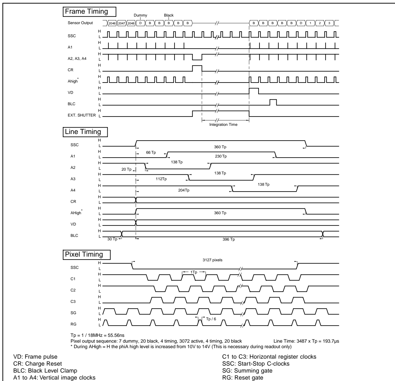
Figure 3 - Timing diagrams
